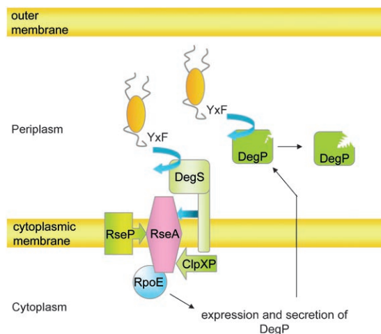
Figure 3. Amplification of bacterial stress response by allosteric activation. DegS senses unfolded proteins and initiates a proteolytic cascade that leads to elevated expression of DegP. In addition, these activating sequences also lead to an allosteric activation of DegP, causing an amplification of the original stress signal by transcriptional and allosteric activation.
