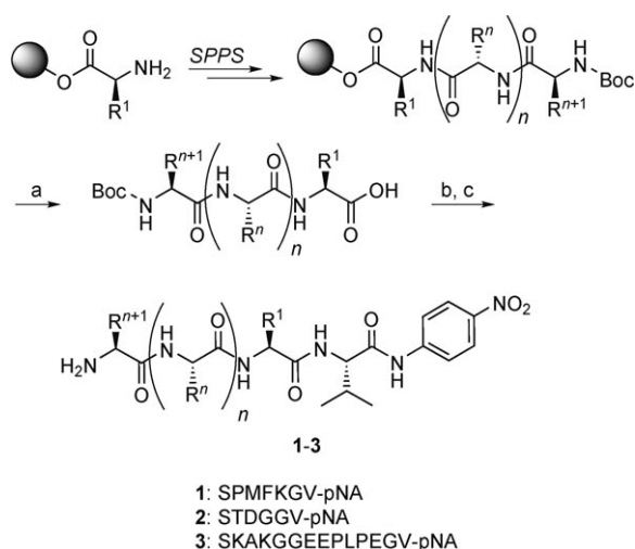
Scheme 1. Synthesis of chromogenic substrates by solid-phase synthesis on 2-chlorotrityl resin. a) Acetic acid/trifluoroethanol/ \text{CH}_2\text{Cl}_2 (2:2:6); b) H-Val-pNA-HCl (2 equiv), EDC-HCl (1.5 equiv), HOBT (2 equiv), DIEA (3.5 equiv); c) TFA/ \text{H}_2\text{O} /ethanedithiol/triisopropylsilane (94:2.5:2.5:1). Boc = tert -butoxycarbonyl, EDC = N -(3-dimethylamino-propyl)- N -ethylcarbodiimide, HOBT = 1-hydroxy-1 H -benzotriazole, DIEA = N,N -diisopropylethylamine, TFA = trifluoroacetic acid.
