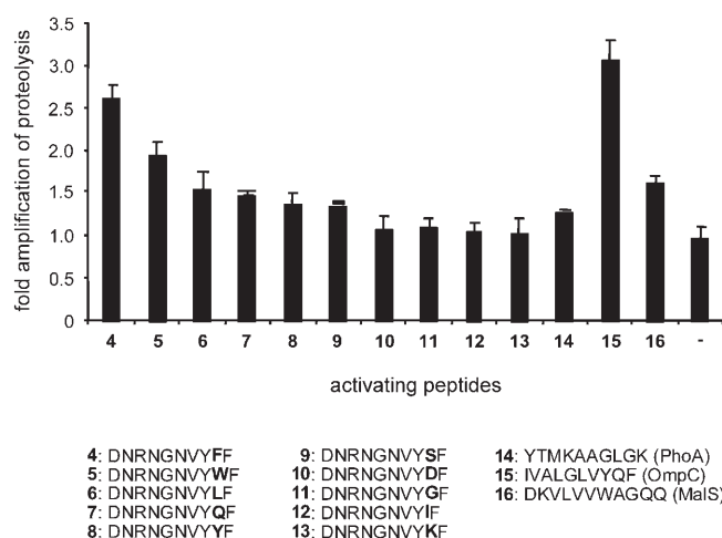
Figure 1. Sequences of activating peptides 4–16 and results derived from proteolysis experiments with 1 . The varied penultimate residue is highlighted in bold. Assay conditions: 0.5 mM 1 , 50 \mu\text{M} activating peptides 4–16 , 0.13 \mu\text{M} DegP, 50 mM \text{NaH}_2\text{PO}_4 pH 8.0 normalized to activity without addition of activating peptide. Each assay was repeated five times with duplicate samples, and the resulting standard deviations are shown as error bars.
