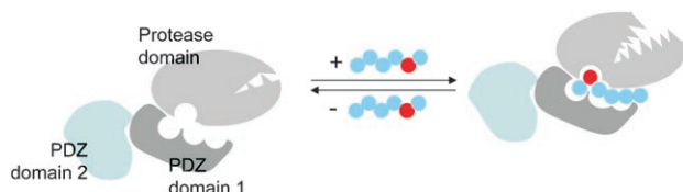
Figure 2. Schematic model of the allosteric activation mode of DegP. Activating peptides (blue circles) bind to PDZ domain 1 and the chemical nature of the penultimate residue (red circle) determines the extent of activation.
